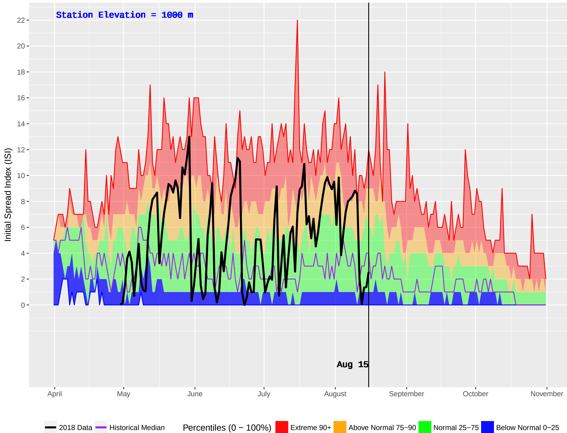
SUCCOUR CREEK (374) : Historical (1986–2016) and Current (2018) Daily Initial Spread Index (ISI)
