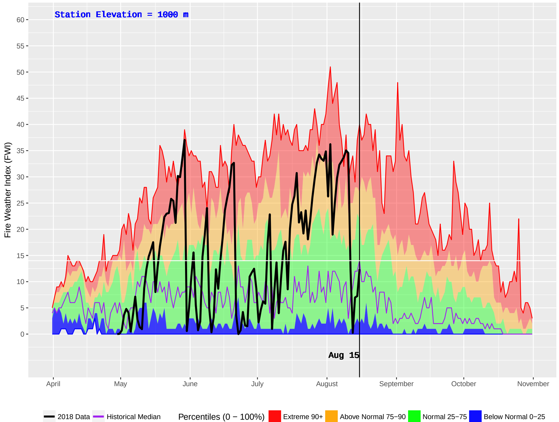
SUCCOUR CREEK (374) : Historical (1986–2016) and Current (2018) Daily Fire Weather Index (FWI)
