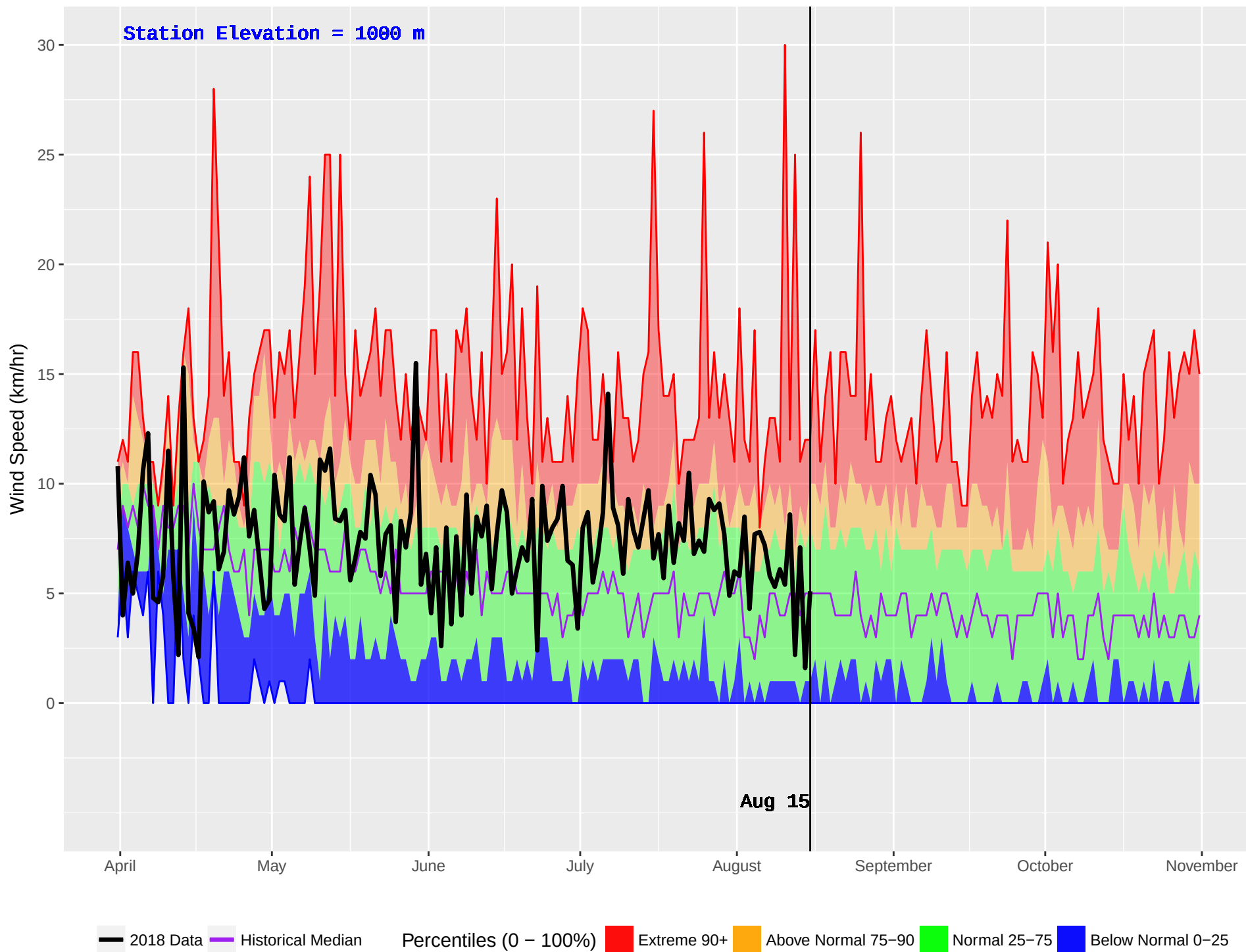
SUCCOUR CREEK (374) : Historical (1986–2016) and Current (2018) Daily Wind Speed
